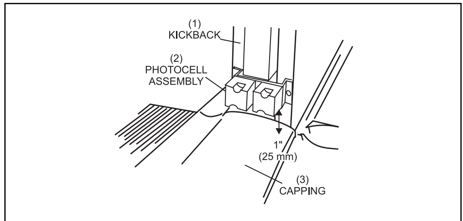
Figure 3-13. Ball Detect.
