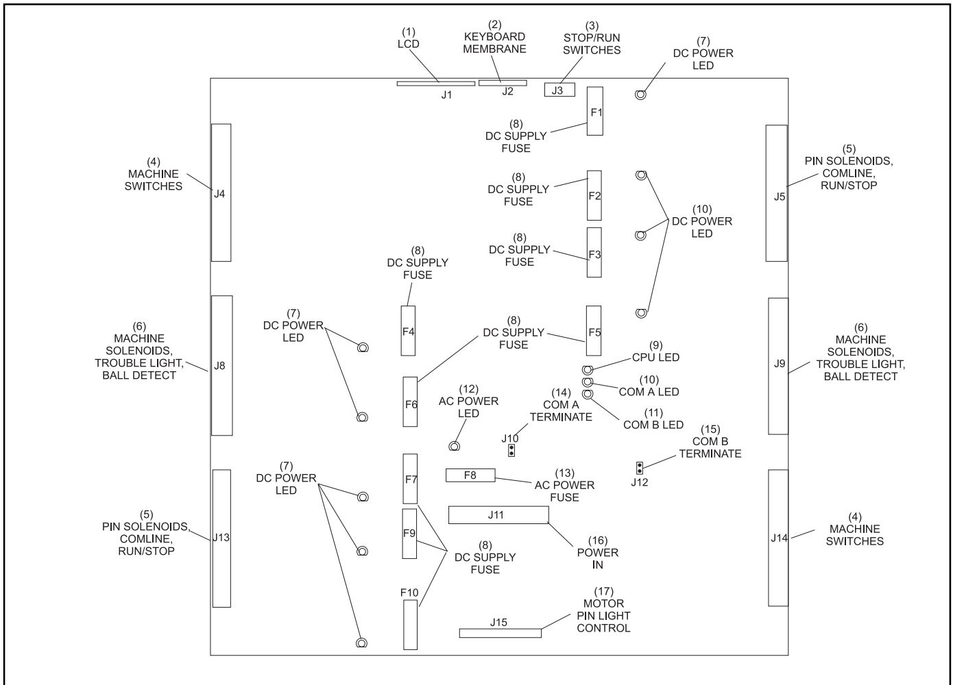
Figure 3-9. CPU PCB.
