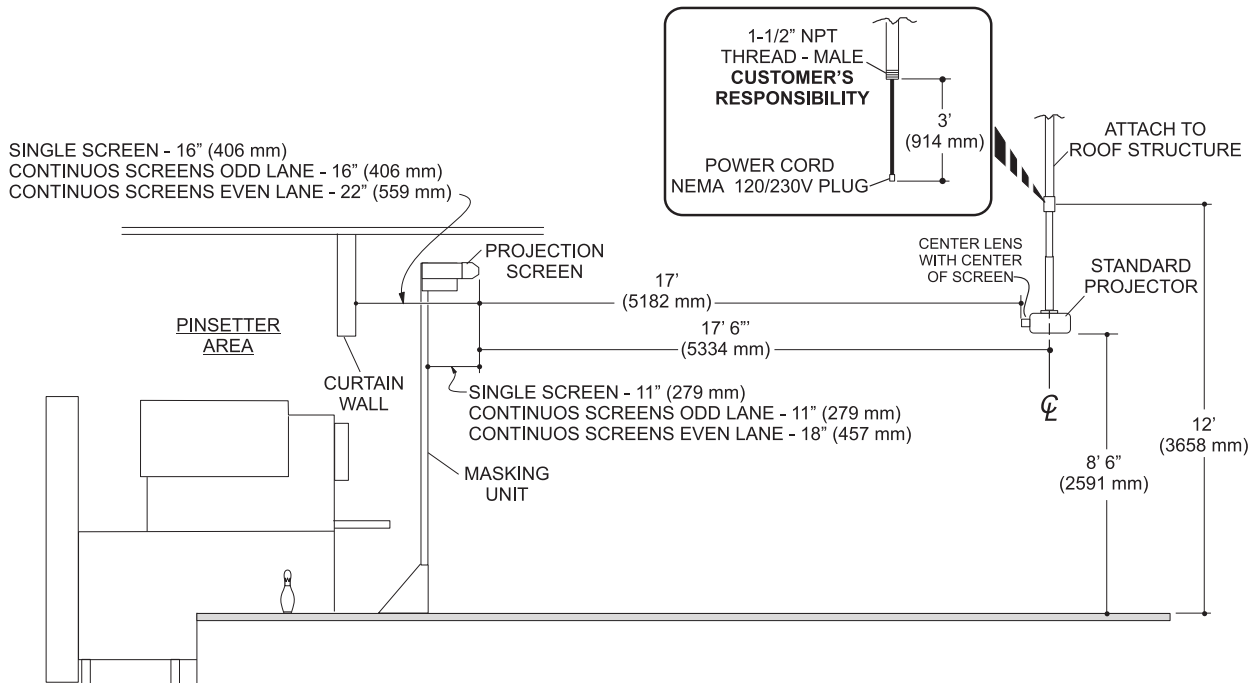
PROJECTION SYSTEM OVERVIEW OPEN CEILING SIDE VIEW
