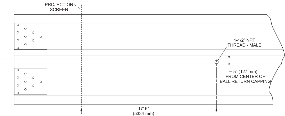
PROJECTION SYSTEM OVERVIEW OPEN CEILING TOP VIEW
